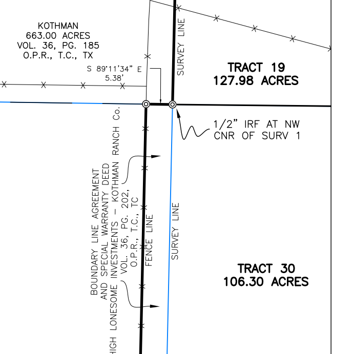
DETAIL No. 4 SCALE 1"=20' STOCK REVOCABLE TRUST 4202.76 ACRES VOL. 255, PG. 72, D.R., T.C., TX
